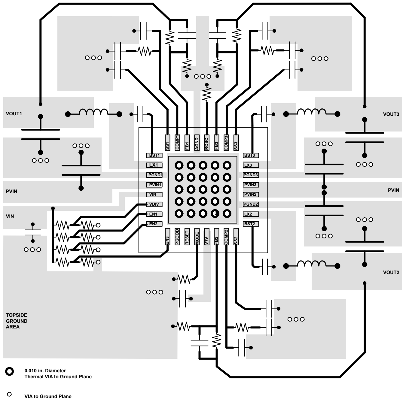
Figure 8-37. PCB Layout
