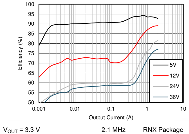
Figure 9-18. Efficiency
