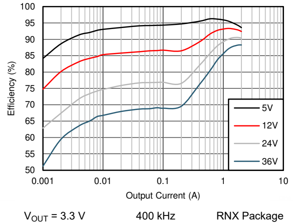
Figure 9-14. Efficiency
