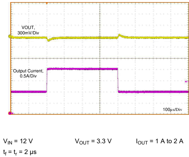
Figure 9-30. Load Transient
