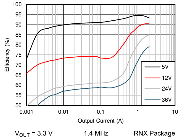
Figure 9-16. Efficiency
