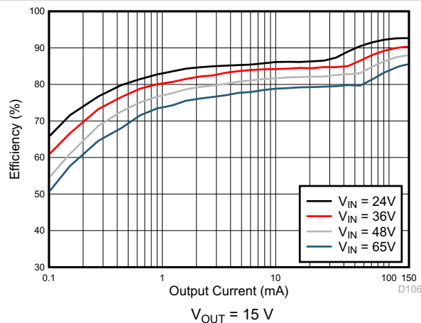
Figure 8-30. Efficiency
