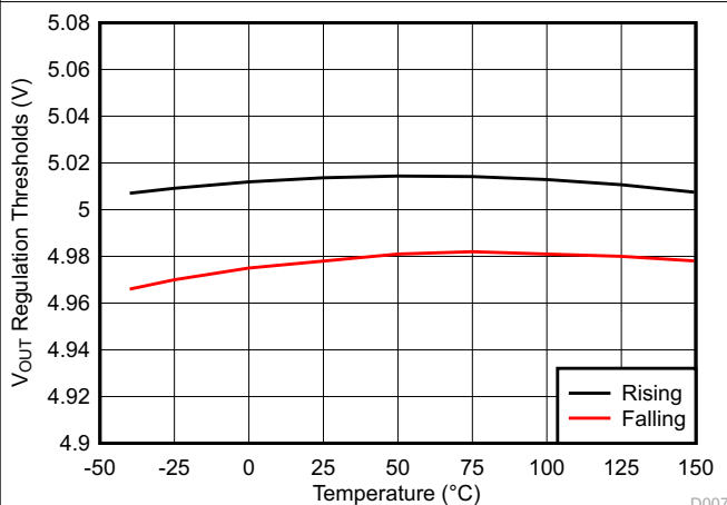
Figure 6-11. VOUT Regulation Thresholds vs Temperature
