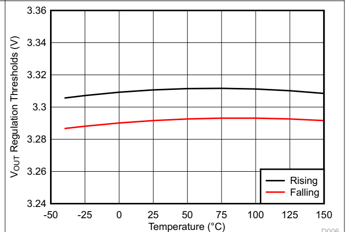
Figure 6-12. VOUT Regulation Thresholds vs Temperature
