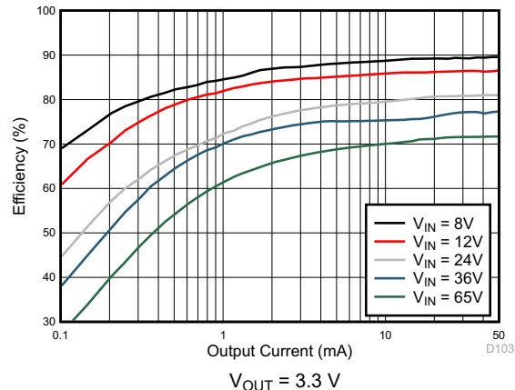
Figure 8-15. Efficiency
