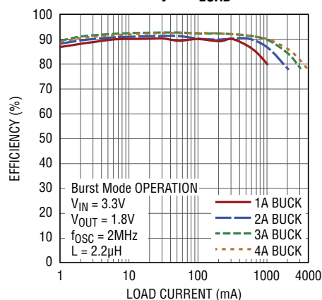
Buck Efficiency vs I_{\text{LOAD}}
