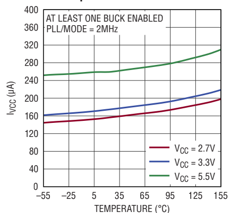
V_{\text{CC}} Supply Current vs Temperature
