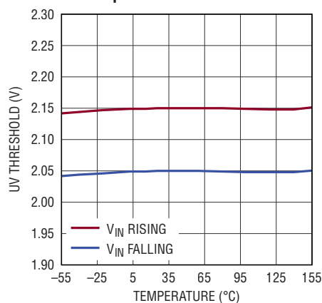
Buck V_{\text{IN}} Undervoltage Threshold vs Temperature
