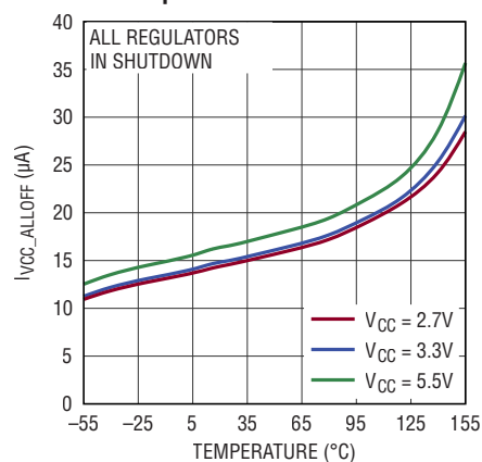
V_{\text{CC}} Supply Current vs Temperature
