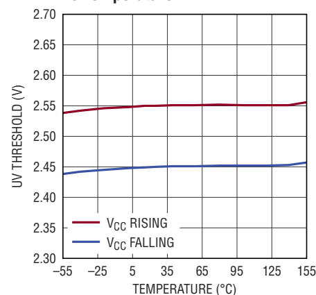
V_{\text{CC}} Undervoltage Threshold vs Temperature
