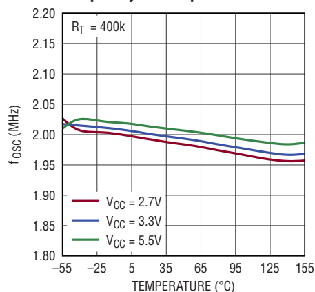
R_{\text{T}} Programmed Oscillator Frequency vs Temperature
