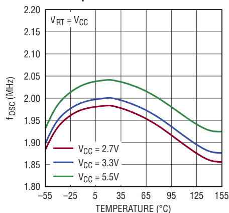
Default Oscillator Frequency vs Temperature
