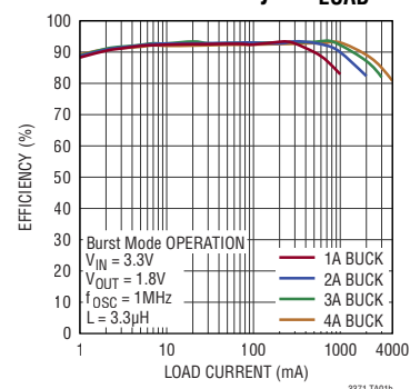
Buck Efficiency vs I_{LOAD}
