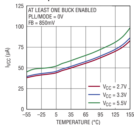
V_{\text{CC}} Supply Current vs Temperature
