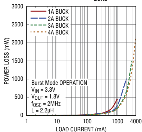
Buck Power Loss vs I_{\text{LOAD}}
