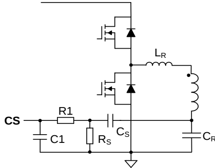
Figure 37: Lossless Current-Sensing Network
