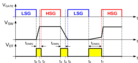
Figure 34: Minimum, Maximum, and Adaptive Dead Time
