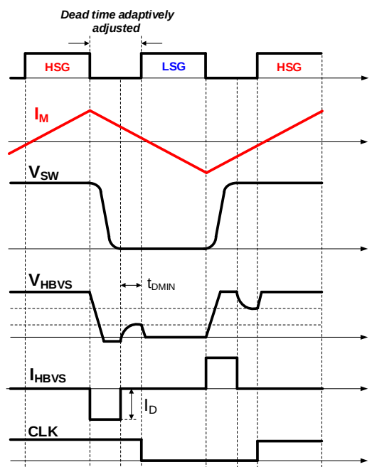
Figure 33: ADTA Operation Waveform
