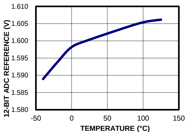
12-Bit ADC Reference vs. Temperature
