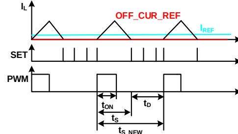
Figure 20: VF-DCM Control Signals
