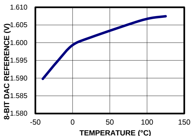
8-Bit DAC Reference vs. Temperature
