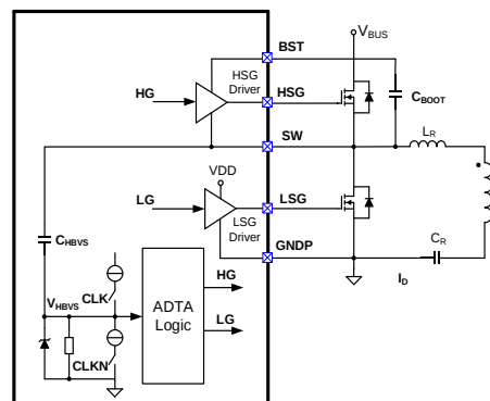
Figure 32: ADTA Block Diagram
