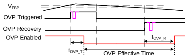
Figure 14: Output OVP
