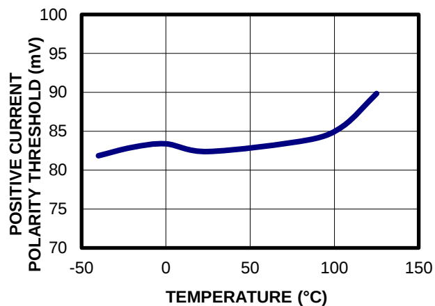
Positive Current Polarity Threshold vs. Temperature
