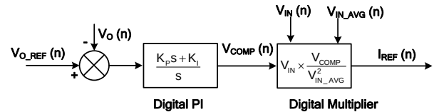
Figure 18: Current Reference
