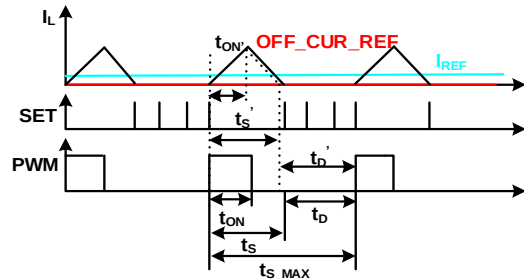
Figure 21: CF-DCM Control Signals
