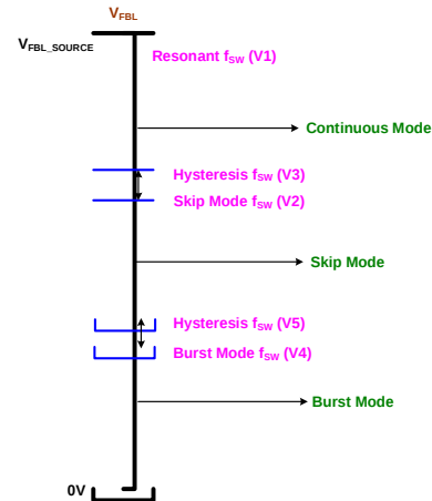
Figure 27: LLC Working Mode Determined by FBL
