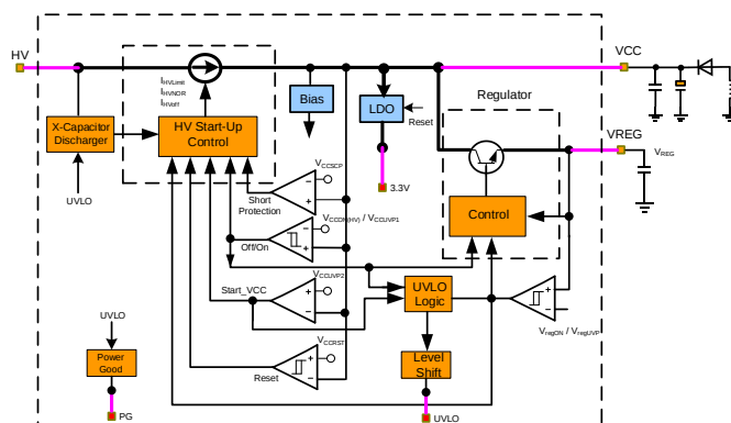
Figure 3: Power Supply Block Diagram
