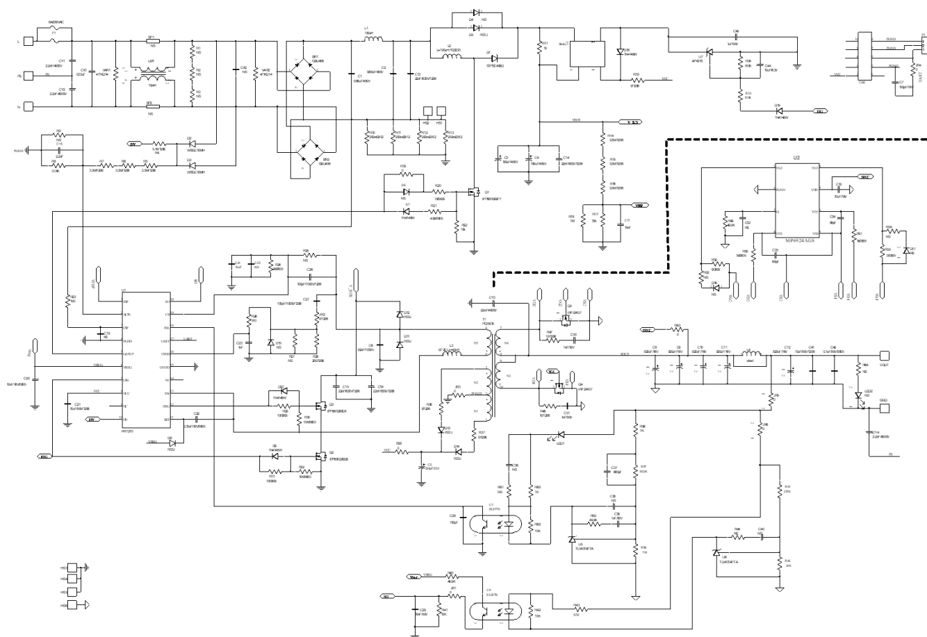
Figure 43: 90-265 V AC Input and 12V/34A Output Application
