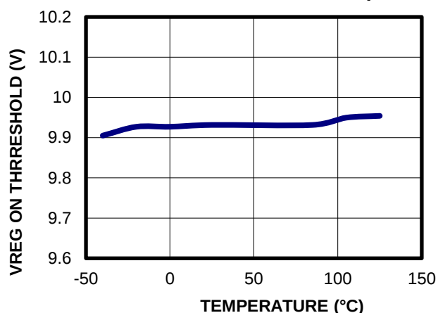
VREG On Threshold vs. Temperature
