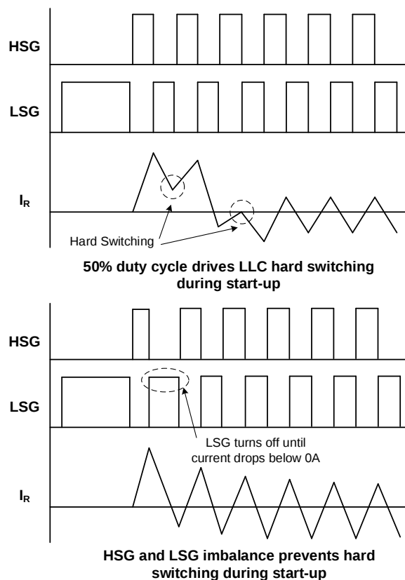
Figure 24: LLC Start-Up to Avoid Hard Switching
