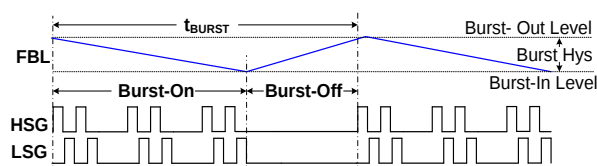
Figure 30: Burst Mode LLC Operation
