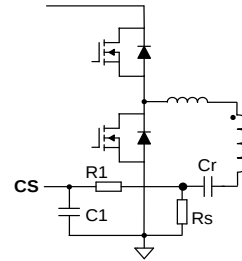
Figure 38: Current Sensing with a Sense Resistor
