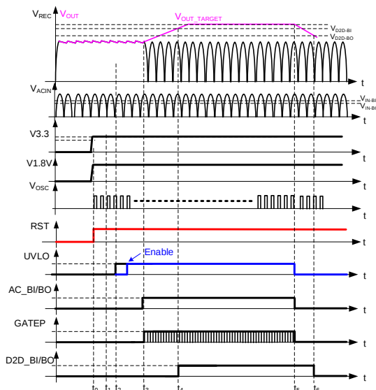
Figure 7: Digital PFC Block Power Supply Timing Sequence
