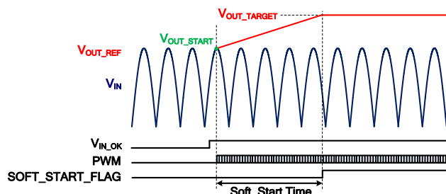
Figure 22: Soft-Start Sequence
