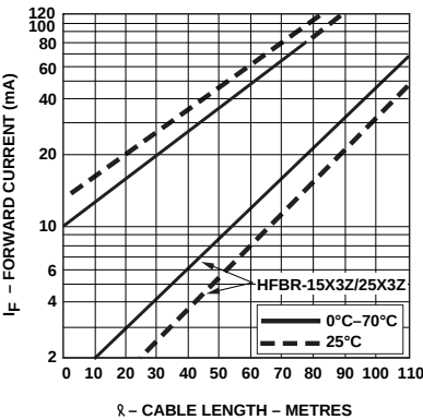
Figure 22. Guaranteed system performance with improved cable.
