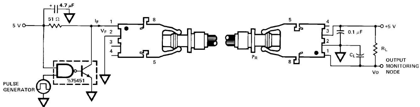
Figure 5. MBd propagation delay test circuit.
