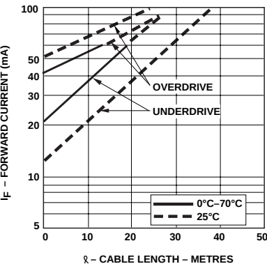
Figure 3. Guaranteed system performance with standard cable (HFBR-15X1Z / 25X1Z).
