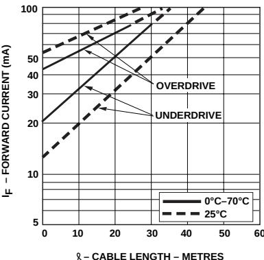
Figure 4. Guaranteed system performance with improved cable (HFBR-15X1Z / 25X1Z).
