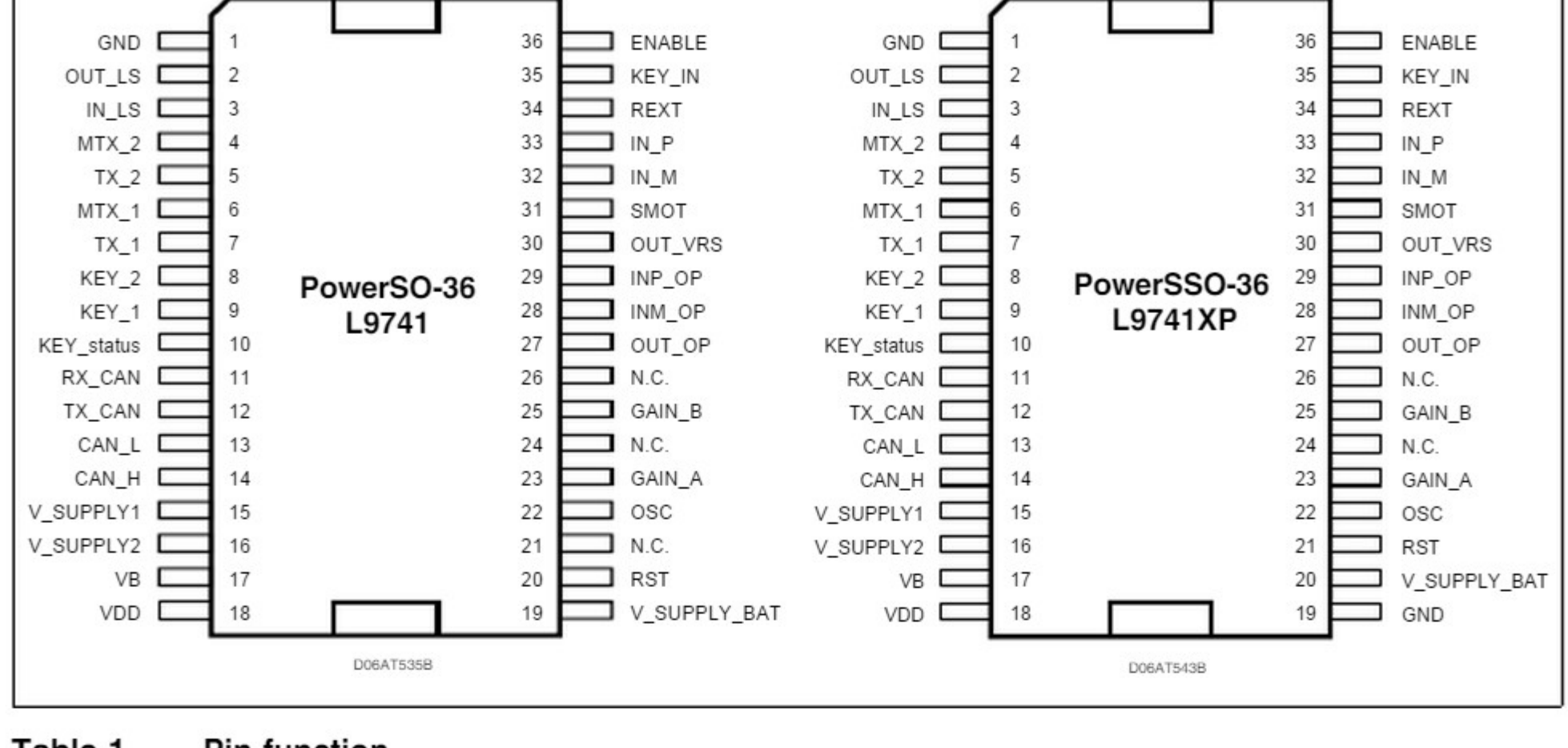
Figure 1. Pins connection (Top view)
