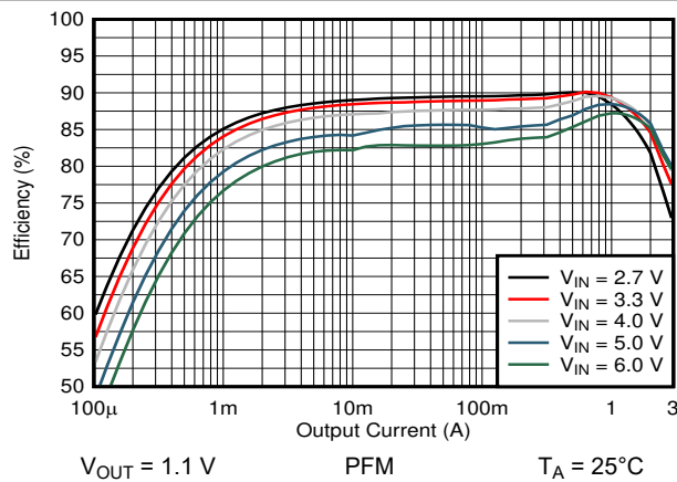
Figure 9-6. Efficiency vs Output Current
