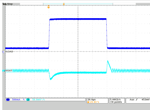
Figure 9-28. Load Transient Response
