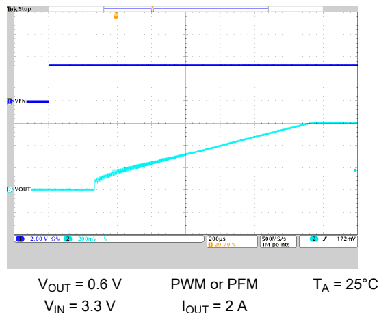
Figure 9-56. Start-Up Timing
