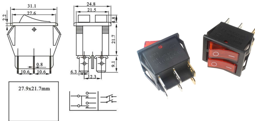
KCD4 AC 250V 16A Red Green Light 6P Terminals ON/Off Double SPST 2 Way Snap in Boat Rocker Switch
