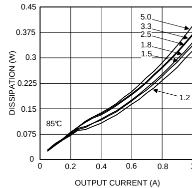
Figure 20. Dissipation 8-V Input at 85°C
