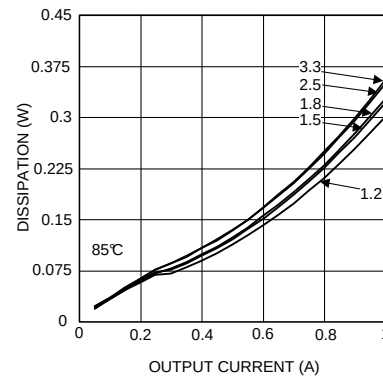
Figure 16. Dissipation 5-V Input at 85°C
